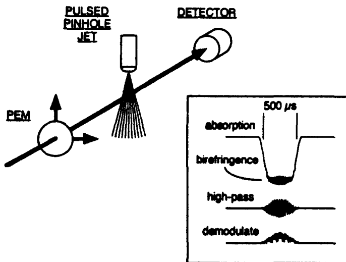
Fig. 5. Apparatus schematic for measuring rotational alignments
